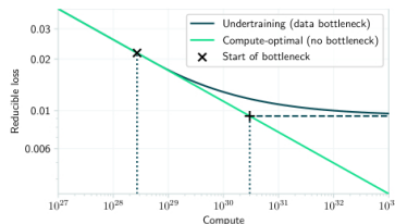
Figure 11: A toy model of undertraining in a data bottleneck scenario in which the stock of data is fixed at 300T tokens. The value of the loss is predicted using the parametric scaling law from Hoffmann et al. (2022), with the revised parameter estimates from Besiroglu et al. (2024). The compute-optimal training compute corresponding to a dataset size of 300T tokens is shown in the left-most black vertical line. We also plot compute-optimal scaling with unlimited data for comparison.
