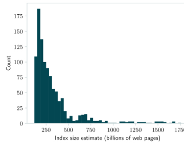
Figure 8: Histogram of the estimates of the size of Google’s index from each pivot word.
